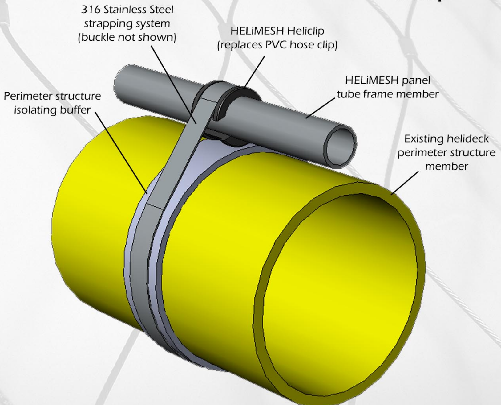
HELIMESH™ Heliclip
